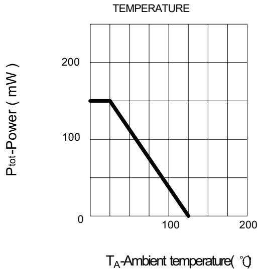
FIG.1--ADMISSIBLEPOWERDISSIPATIONVS. AMBIENT
